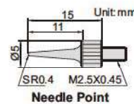
Needle Point
