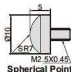
Spherical Point
