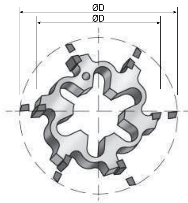
The cutting rings can be expanded for recovering the starting diameter.
